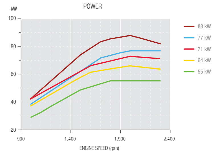
MF 3 SPECIALITY SERIES - POWER & TORQUE CURVES
